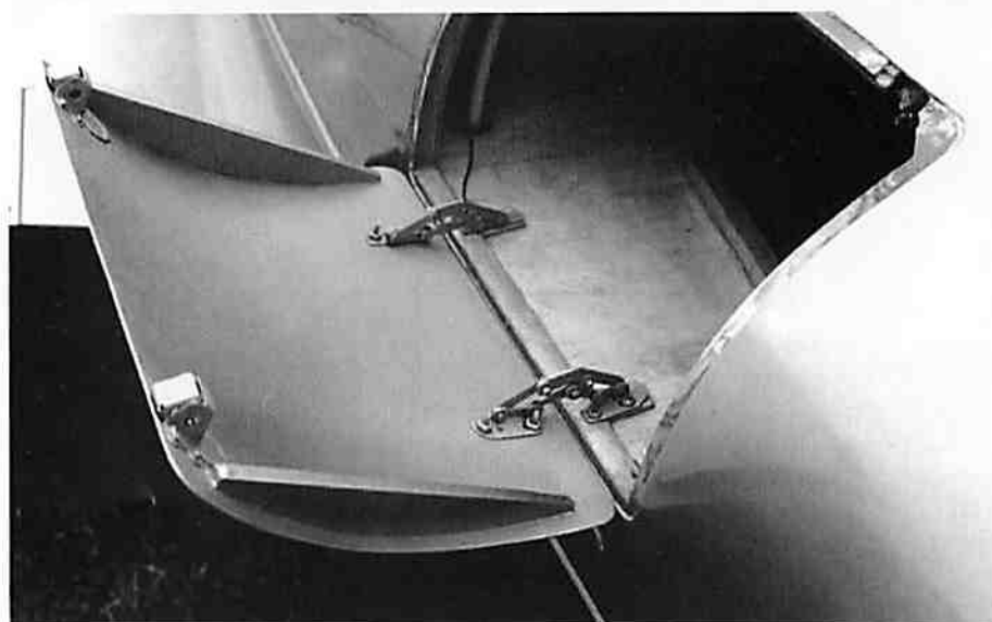
Top: Down-limit switch on George Barrett's Falco.
